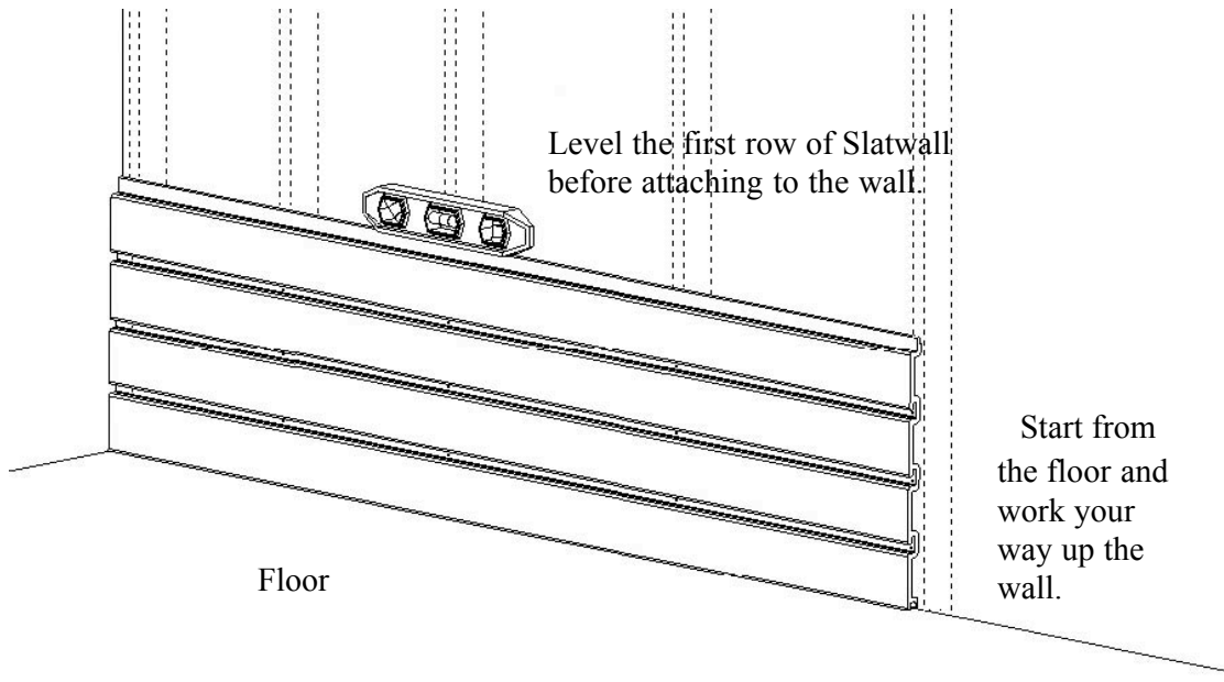
Figure 1. Level SLATWALL before attaching it to the wall
